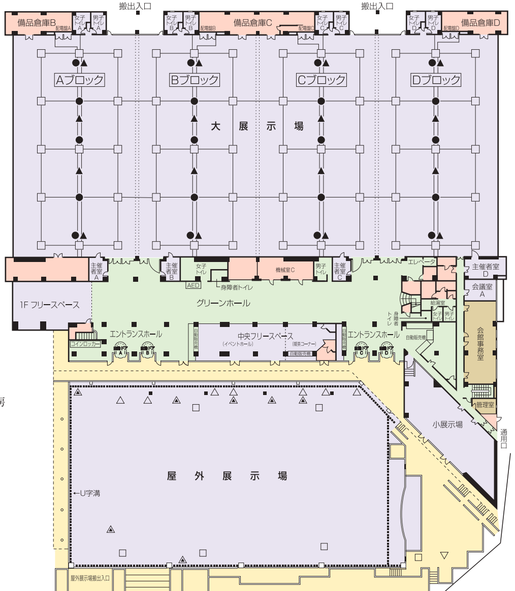
[1階平面図]
